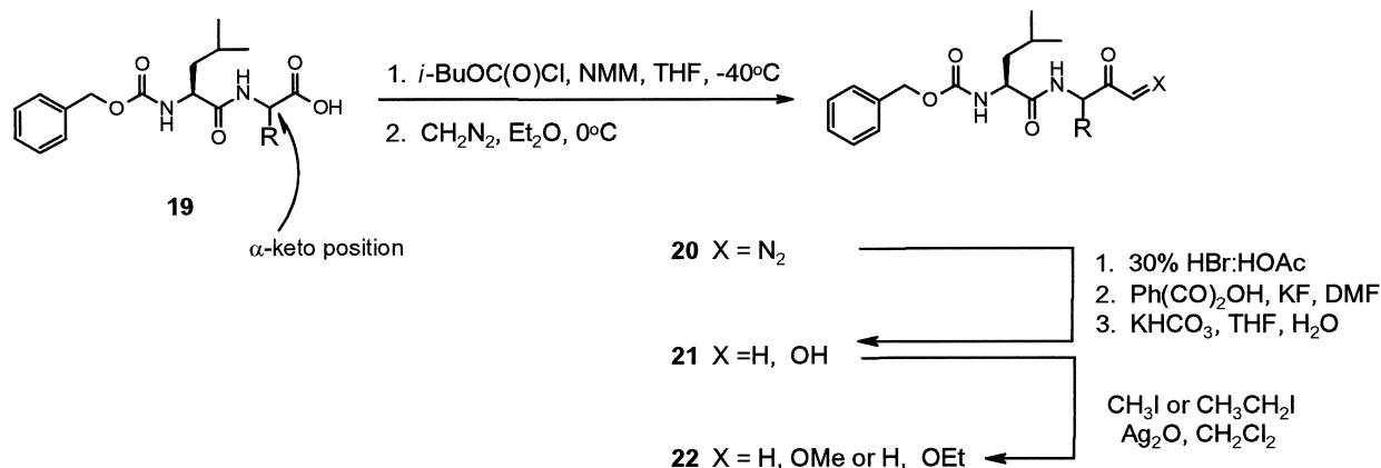
Scheme 2. Synthesis of P2 modified alkoxy methylketone inhibitors.
