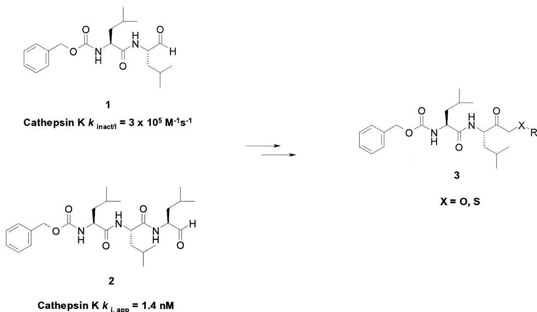
Figure 1. The evolution of the alkoxyethylketone and thiomethylketone cathepsin K inhibitors 3 from the aldehyde inhibitors 1 and 2 .
