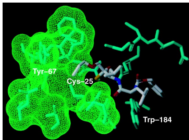
Figure 2. View of the X-ray co-crystal structure of inhibitor 8 (white) bound in the active site of cathepsin K (blue). Cysteine 25 (yellow) is attached covalently to the carbonyl group of the inhibitor forming a hemi-thioether. The n -propyl ether slightly penetrates the P2 pocket of the enzyme. The phenyl group of the Cbz is bound in the P3' pocket forming a \pi -stacking interaction with Trp184.
